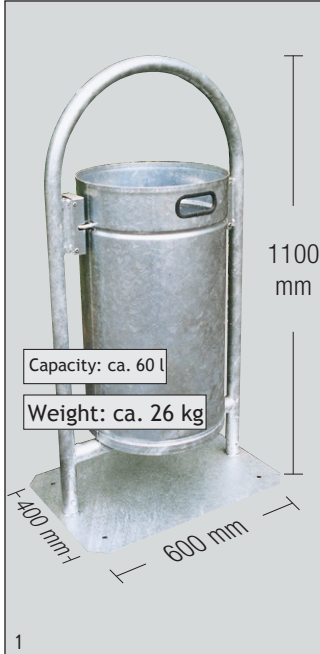
Pic.: RB004, with bottom plate, corpus hot-galvanized, Art.-No. 3002
